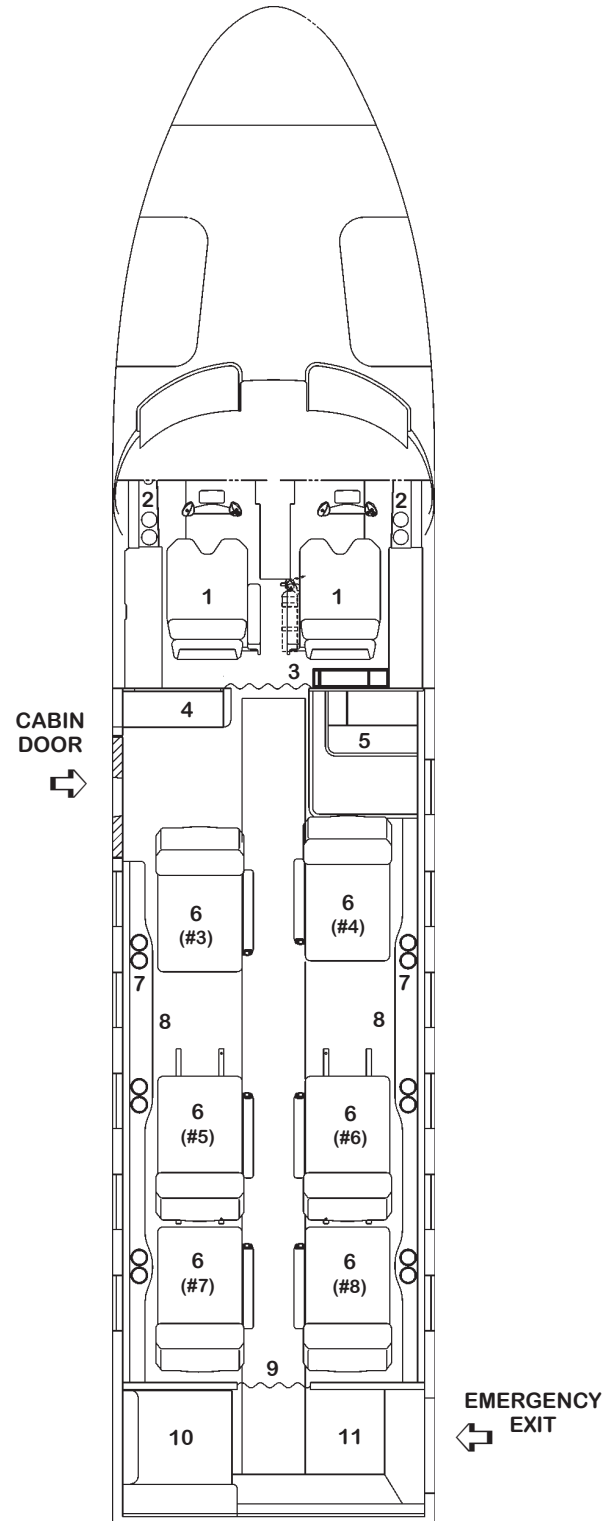
FIGURE IV — CITATION CJ2+ STANDARD FLOORPLAN
