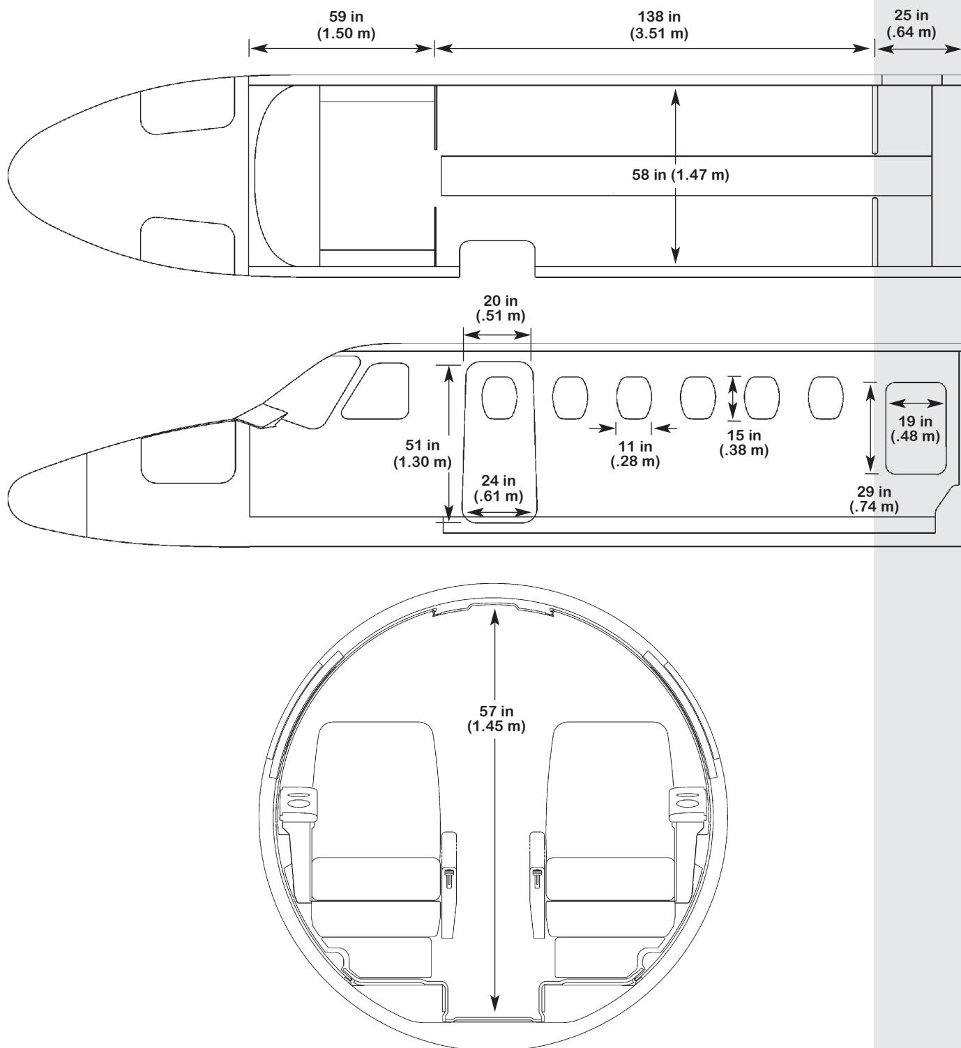
FIGURE II — CITATION CJ2+ INTERIOR DIMENSIONS
