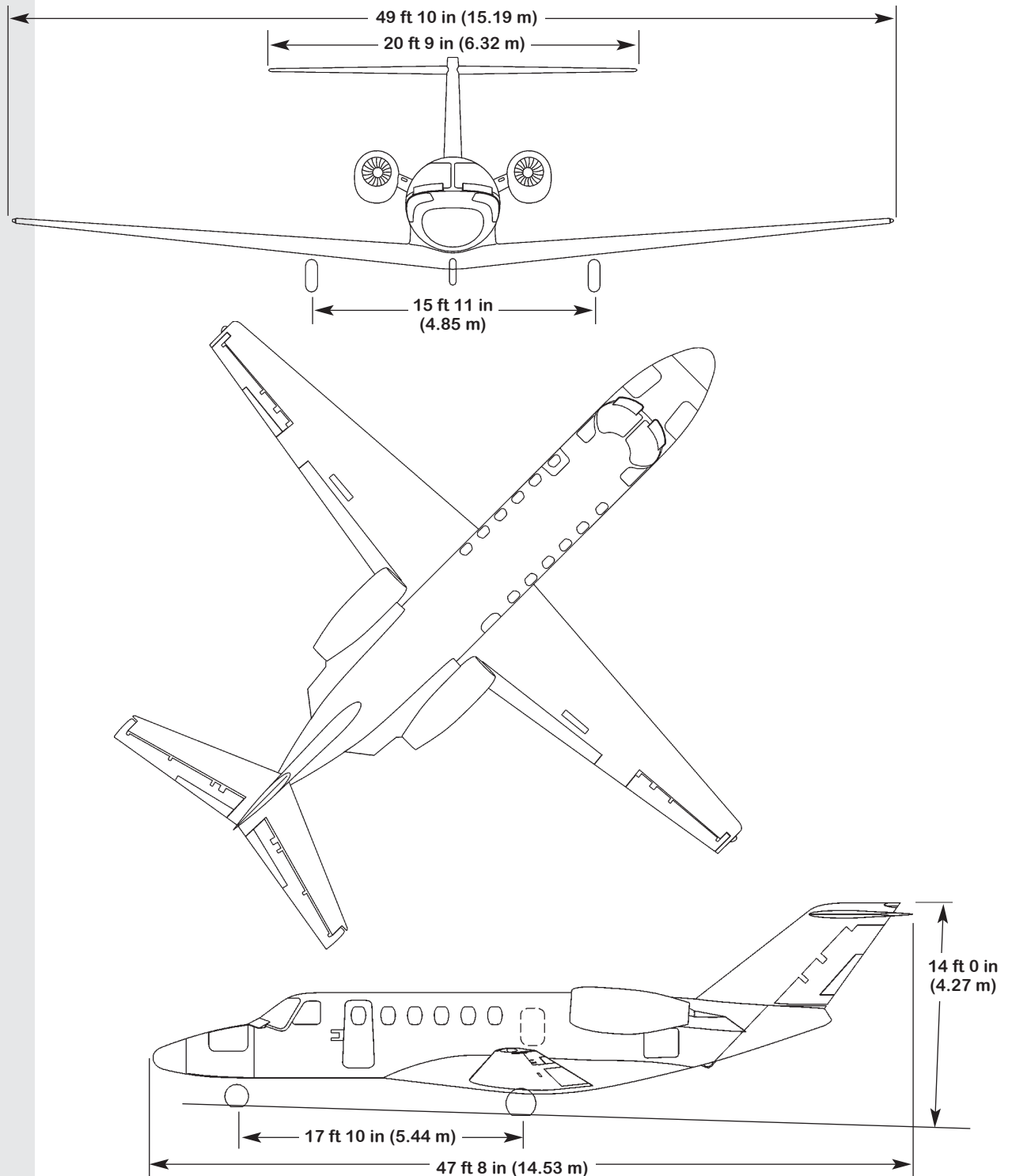
FIGURE I — CITATION CJ2+ EXTERIOR DIMENSIONS
